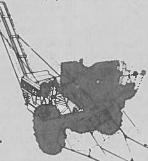
Uni-System picker has giant 12-roll husking bed, biggest on the market. Special presser wheels with 312 moving rubber Flexi-Fingers align the ears and keep them moving along the husking rolls. You get cleaner corn.
